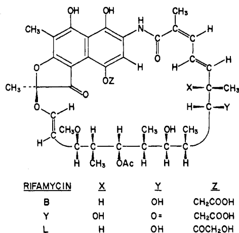
Figure 1. Structures assigned to rifamycins.
