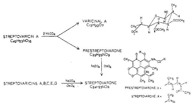
Figure 7. Degradation products derived from the streptovarinins.
